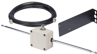
Remote Dipole Antenna MV-ALS-AT02 Operating range: up to 1500 ft. Remote-mounting from Stationary Base Transmitter, mounting kit and 25' coaxial cable included
